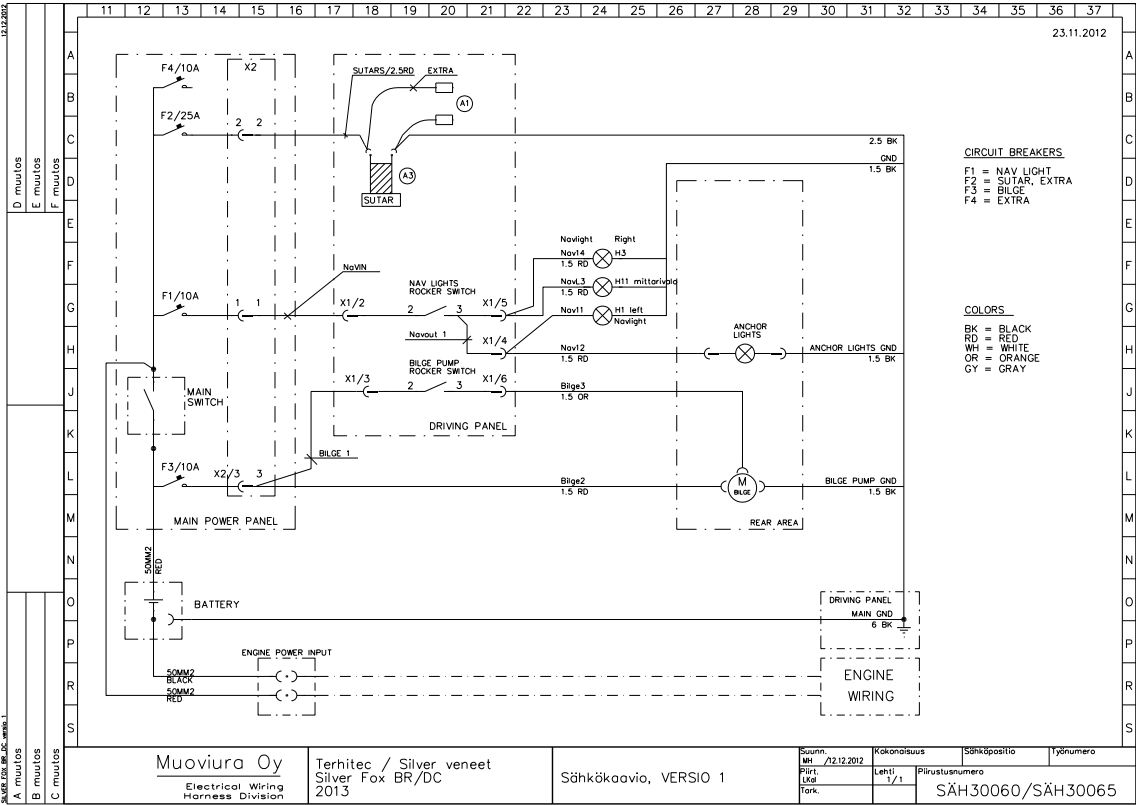
Fig. 5. Electrical diagram
