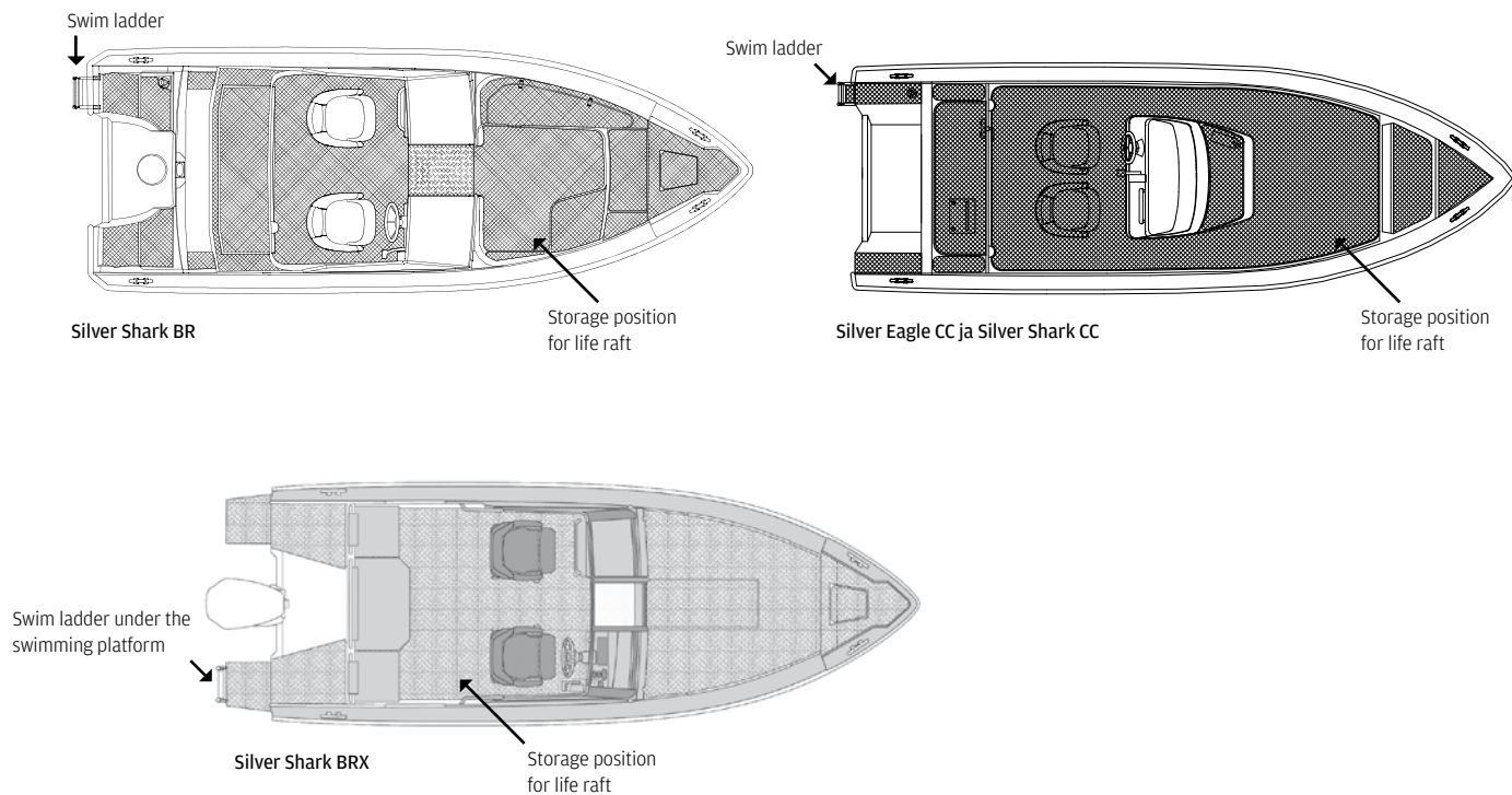
158 Fig. 4. Swim ladder position and anti-slip surfaces. Recommended storage position for life raft.
