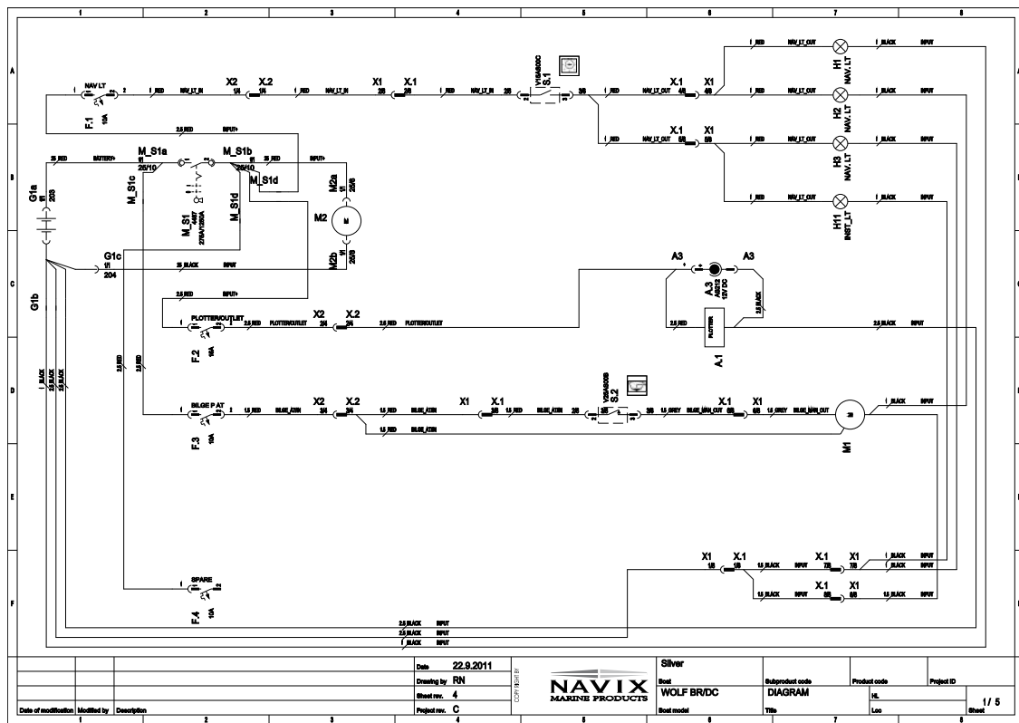
Fig. 5. Electrical diagram
